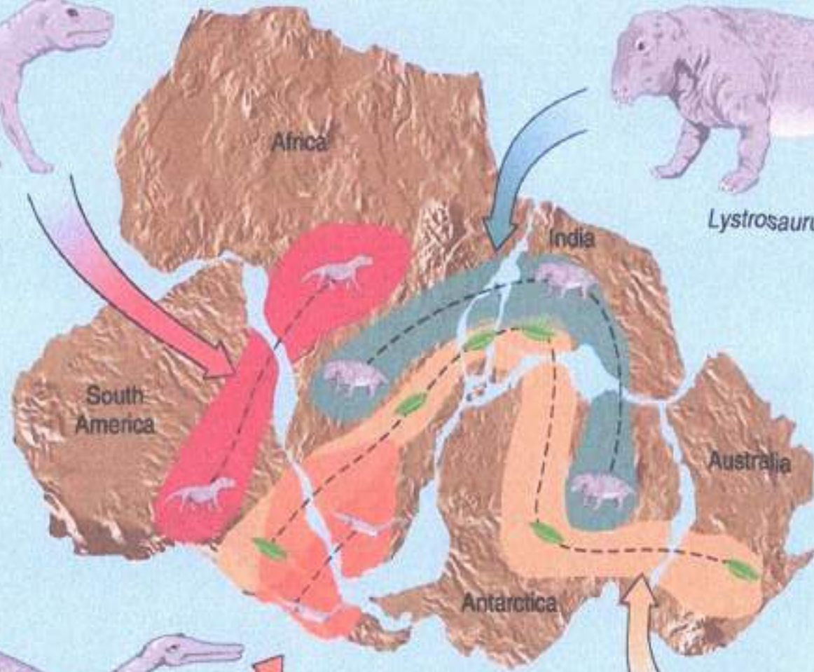
Cynognathus
