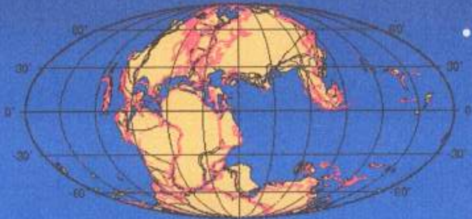
150 My Reconstruction
